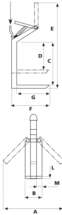
DIMENSIONS (mm):
